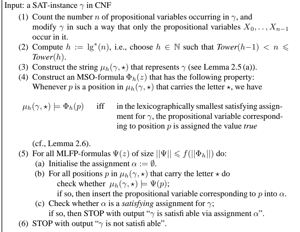
FIGURE 2. A SAT-solving algorithm.
